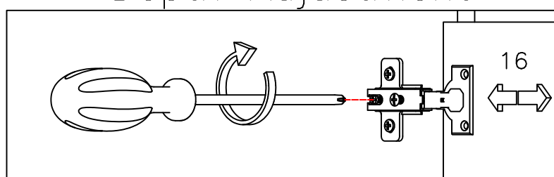
Depth Adjustment
